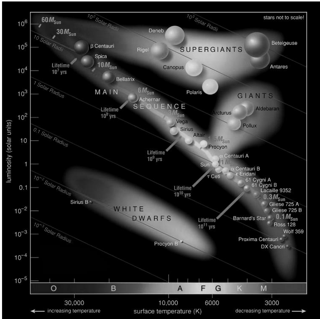
Figure 2: Hertzsprung-Russell diagram.
